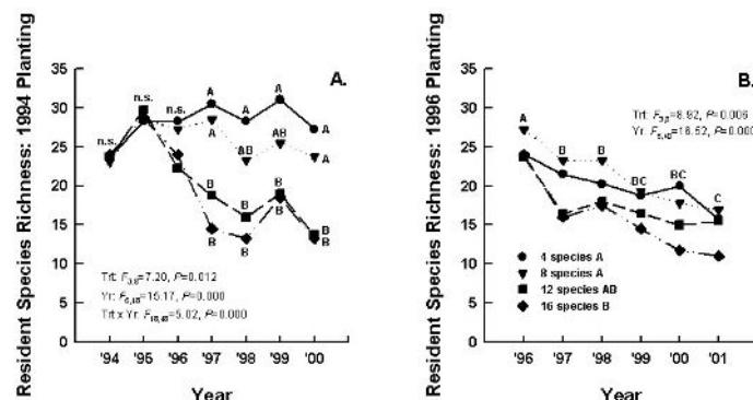
Figure 6. Richness of resident species in 16 plots planted to four richness treatments in A. 1994 and B. 1996. Within each year (A.), symbols with the same letter indicate that means do not differ at P < 0.05 (ANOVA, Tukey's HSD procedure). Treatment designations or years (B.) with the same letter indicate that means do not differ at P < 0.05 (ANOVA, Tukey's HSD procedure).
