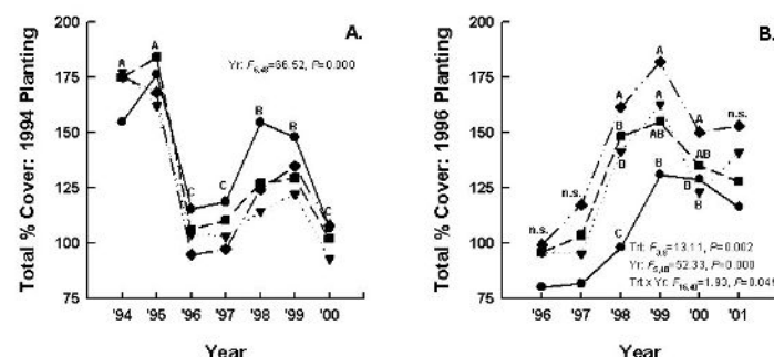
Figure 3. Total percentage cover of 16 plots planted to four richness treatments in A. 1994 and B. 1996. Year designations (A.) with the same letter indicate that means do not differ at P<0.05 (ANOVA, Tukey's HSD procedure). Within a year (B.), symbols with the same letter indicate that means do not differ at P<0.05 (ANOVA, Tukey's HSD procedure).
