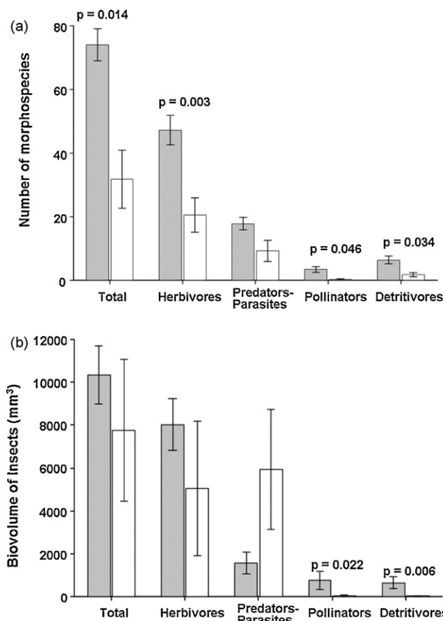
Fig. 3. Means ( \pm 1 S.E.) of insect (a) morphospecies richness and (b) biovolume in perennial grass (shaded bars) and annual wheat (open bars) fields ( n = 5 ). Groups with significantly different means are denoted with respective p -values.
