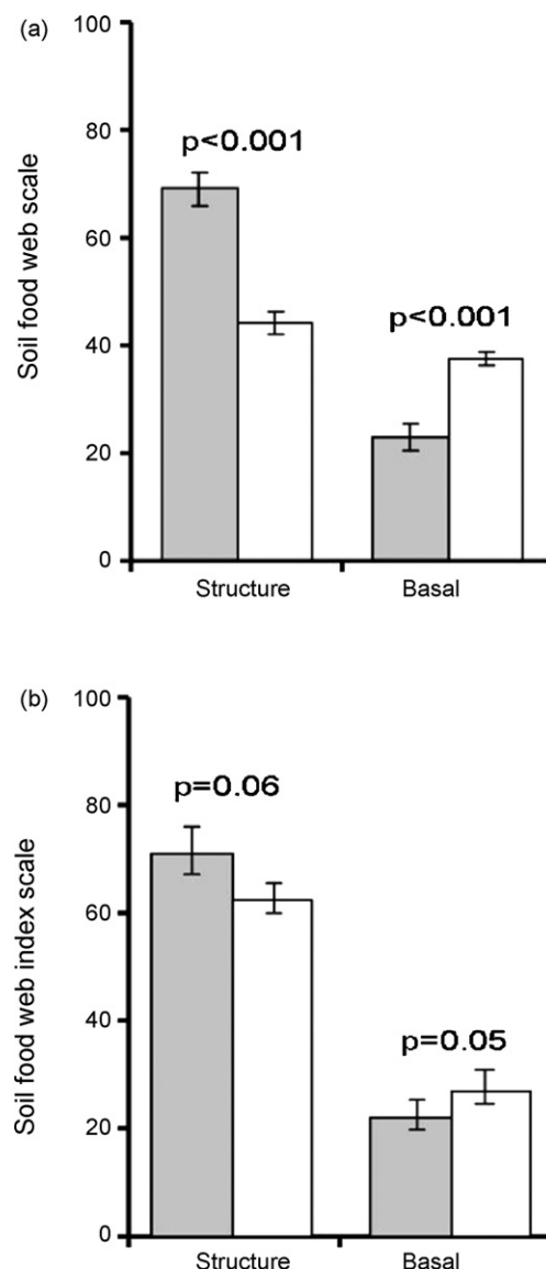
Fig. 5. Nematode community structure indices for perennial grass (solid bars) and annual crop (open bars) fields to a depth of 1 m in (a) long-term study sites ( n = 5 ) and (b) conversion study plots ( n = 3 ). Error bars indicate standard errors of means.
