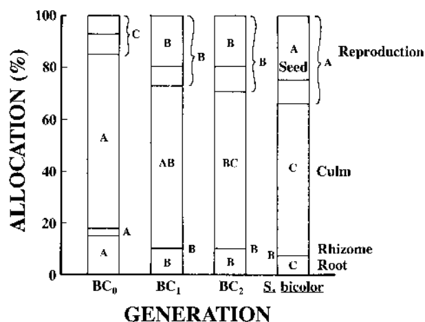
FIG. 2. Mean biomass allocation (%) for Sorghum bicolor and three generations of S. bicolor \times S. halepense crosses. The reproductive portion (panicle) is further divided into seed and accessory reproductive structures (e.g., pedicels). Bar sections with the same letter do not differ at p < 0.05 (ANOVA; Duncan's multiple range test).
