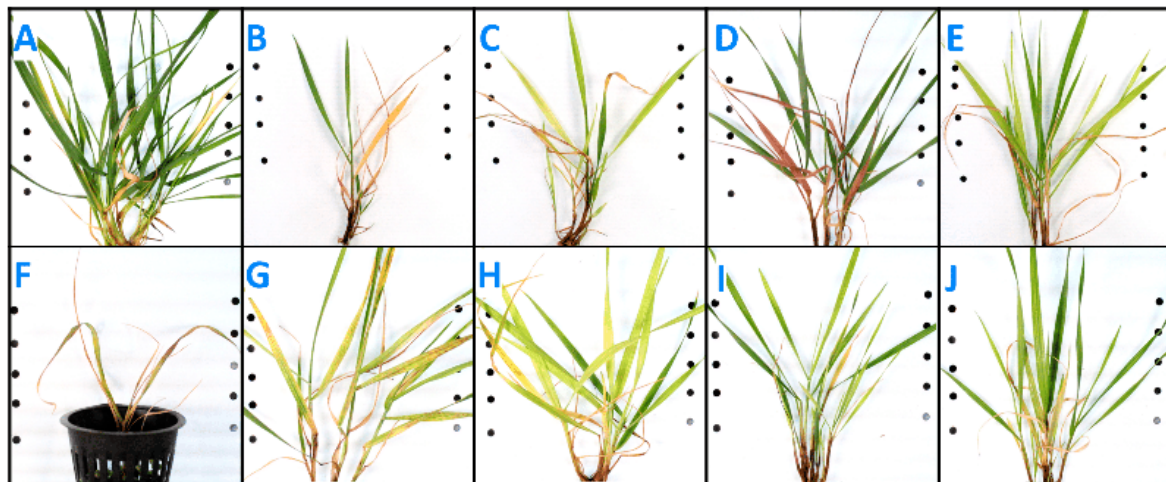
Figure 1. Intermediate wheatgrass aboveground symptoms at 5 weeks post-transplanting into nutrient deficient solution (except calcium—photo taken at 3.5 weeks post-transplanting): (A) control, (B) nitrogen, (C) potassium, (D) phosphorus, (E) sulfur, (F) calcium, (G) magnesium, (H) iron, (I) boron, and (J) zinc.
